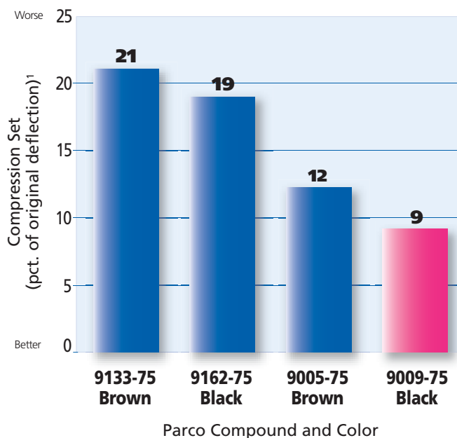
Compression Set of Typical Parco 75-Durometer FKM Compounds
