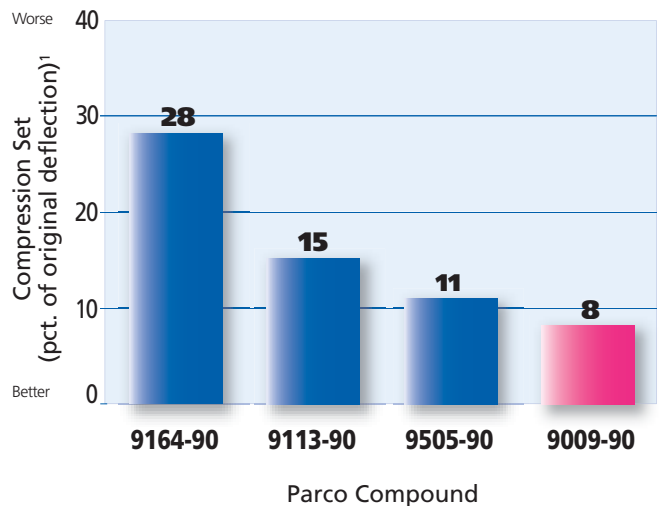
Compression Set of Typical Parco 90-Durometer FKM Compounds
